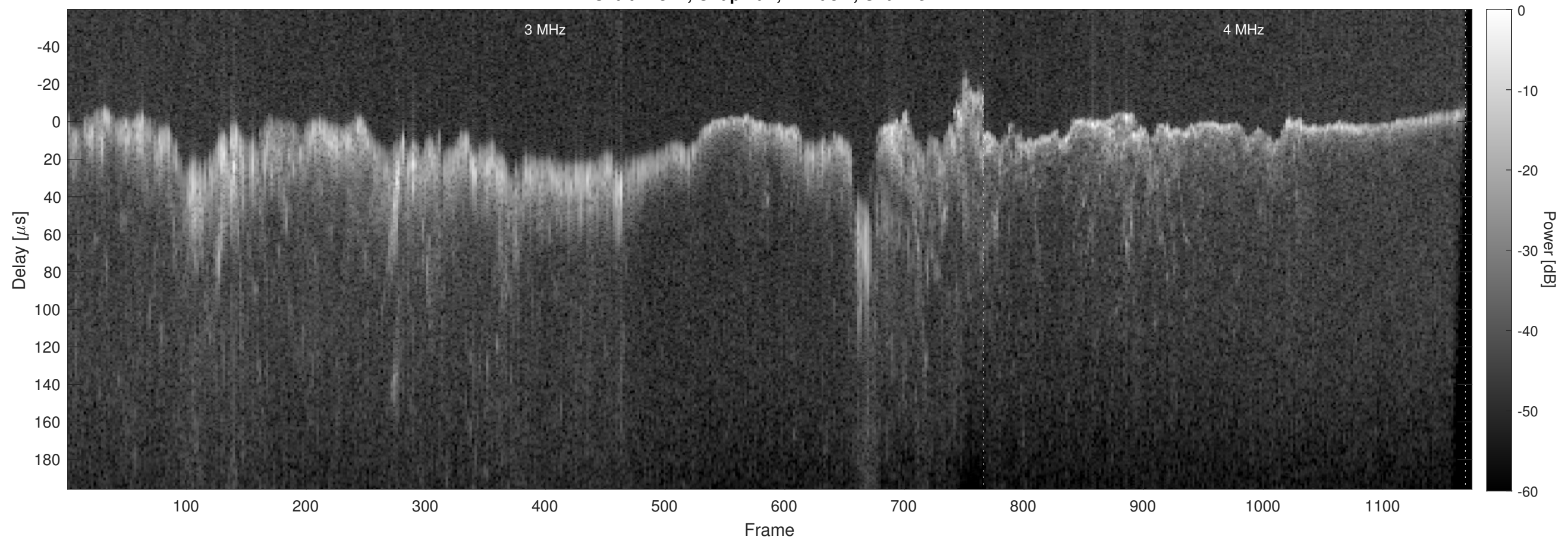
Orbit 12377, Chapman, Window, Channel 2
