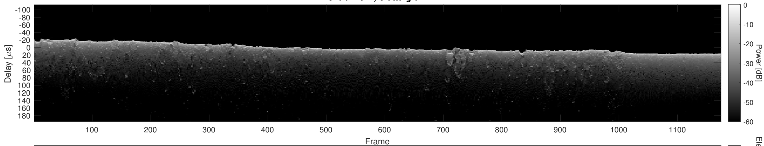
Orbit 12377, Cluttergram
