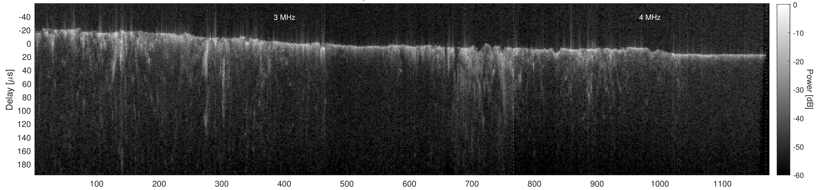
Orbit 12377, Cluttergram
