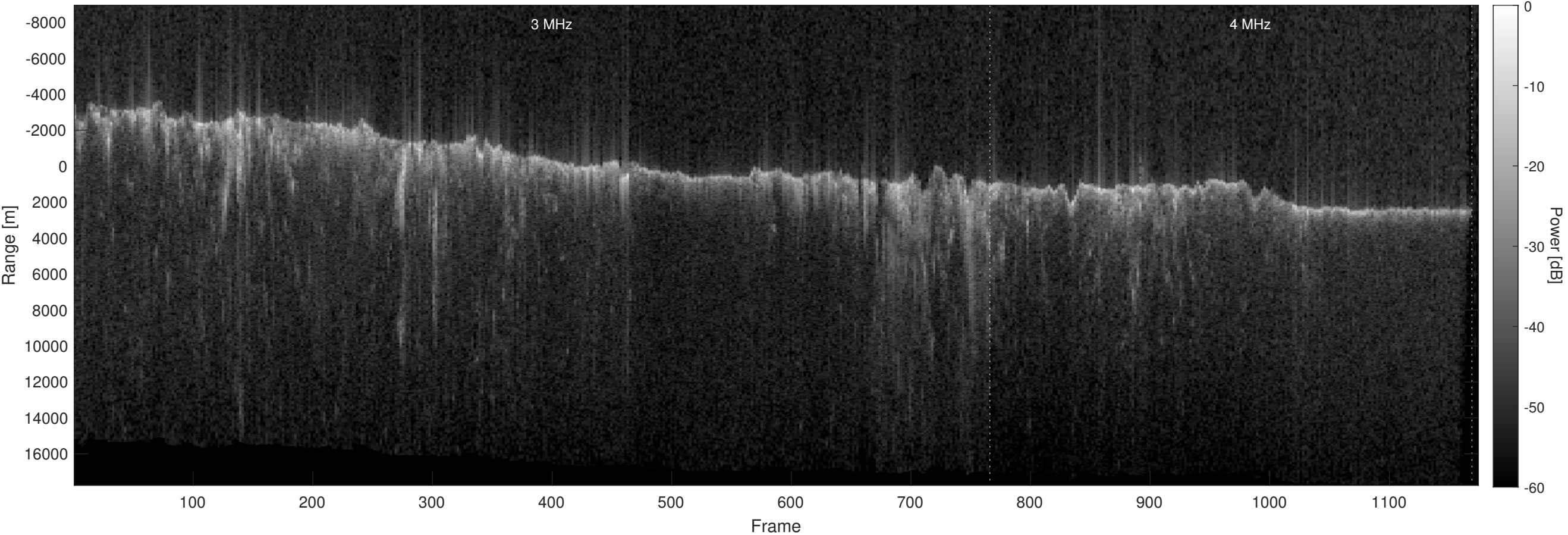
Orbit 12377, Optimized, No Window, Depth-Corrected, Channel 2
