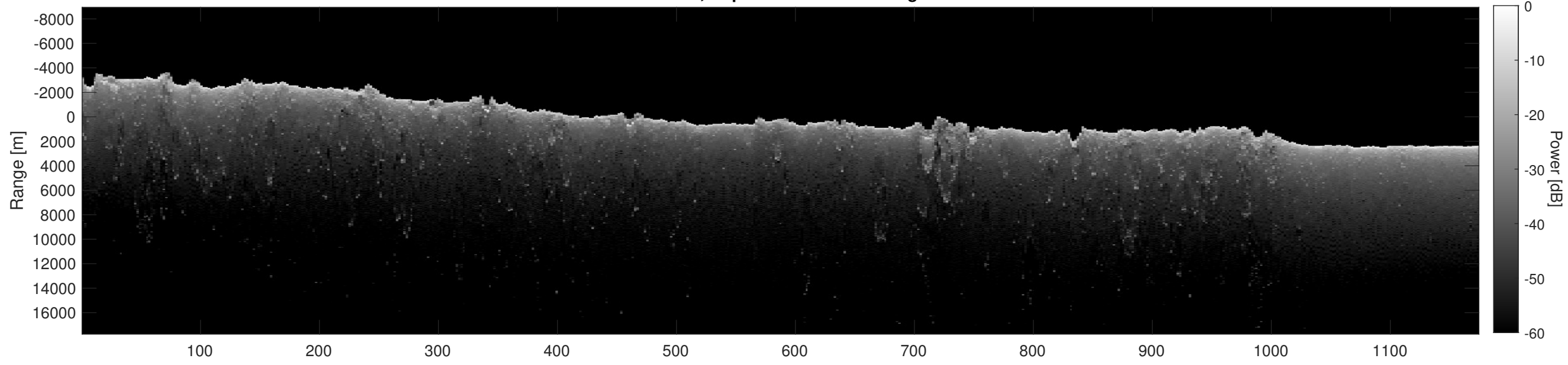
Orbit 12377, Depth-Corrected Cluttergram
