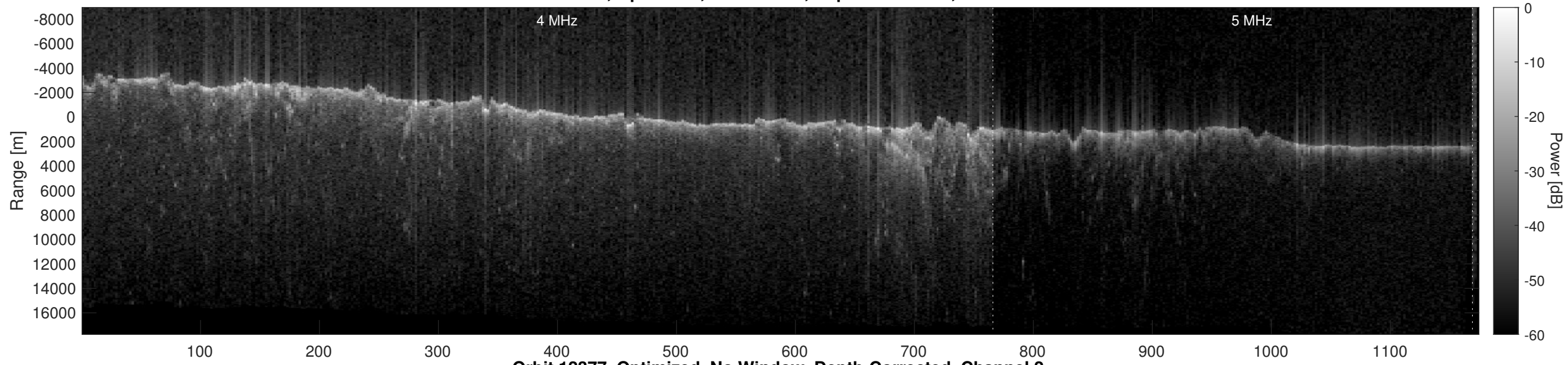
Orbit 12377, Optimized, No Window, Depth-Corrected, Channel 2
