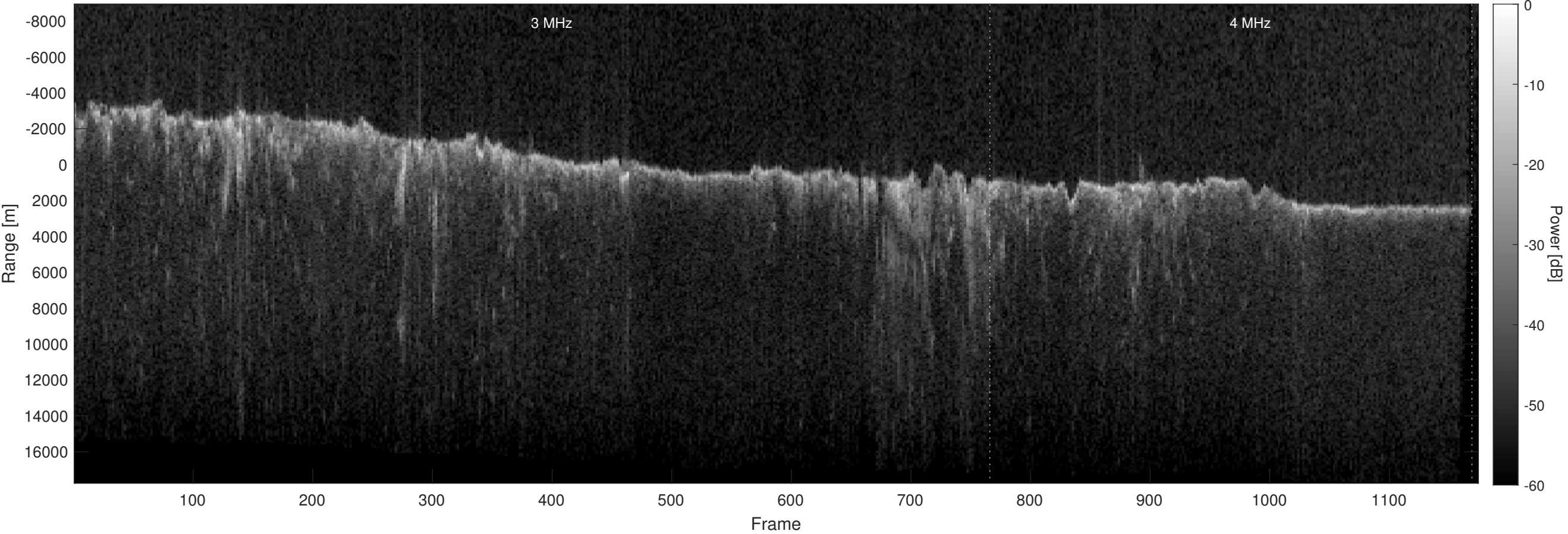
Orbit 12377, Optimized, Window, Depth-Corrected, Channel 2
