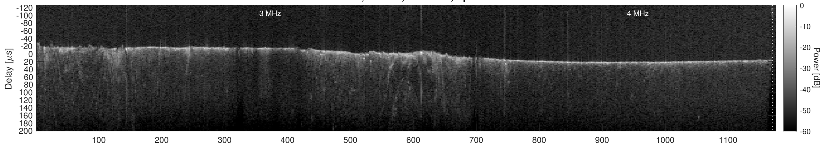
Orbit 12383, Cluttergram
