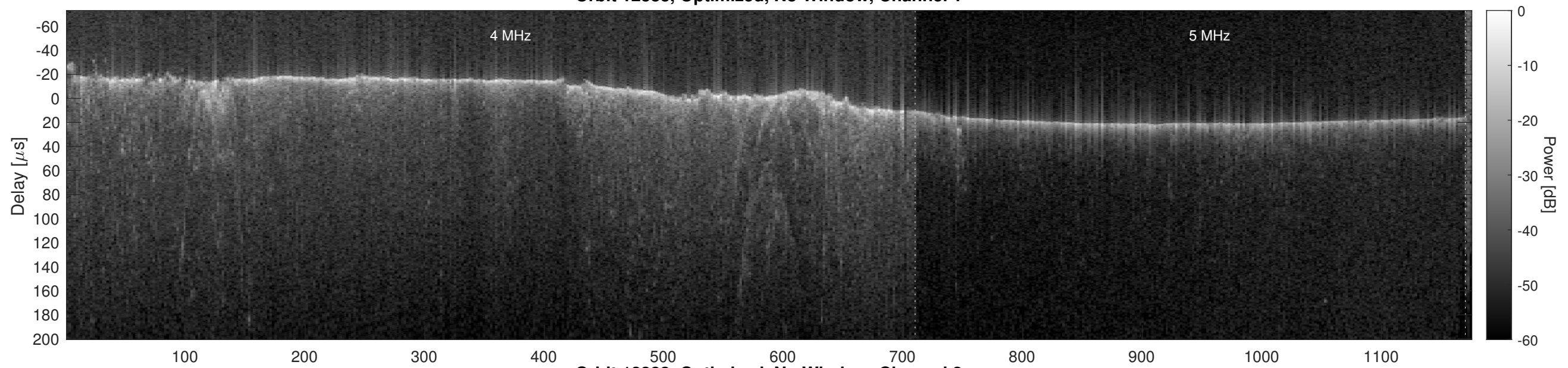
Orbit 12383, Optimized, No Window, Channel 2
