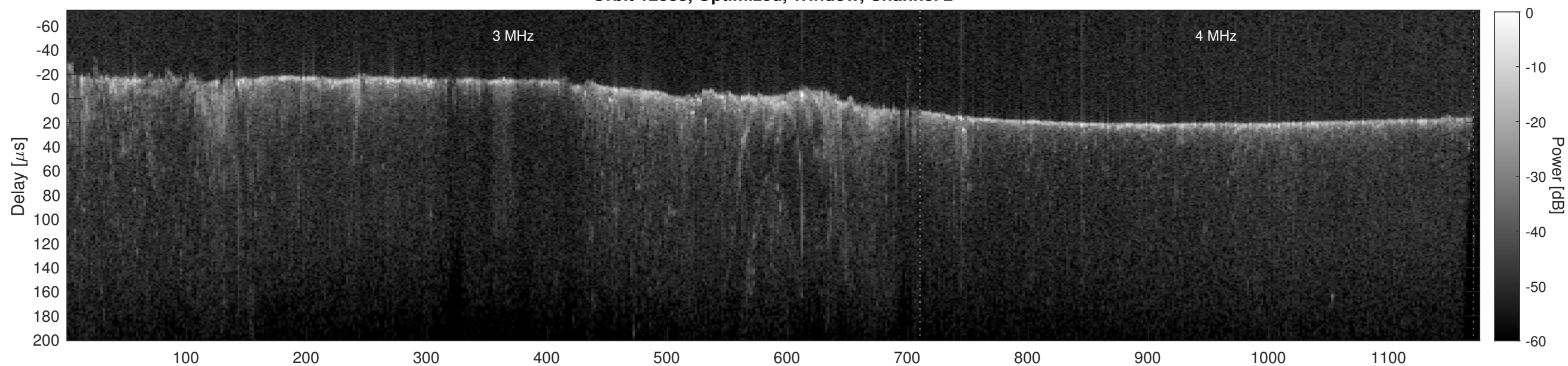
Orbit 12383, Cluttergram
