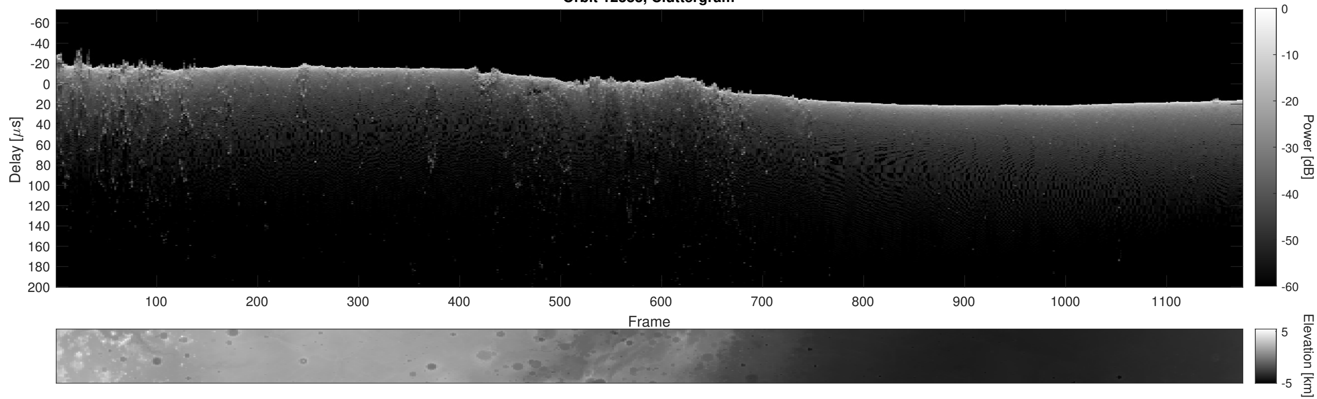
Orbit 12383, Cluttergram
