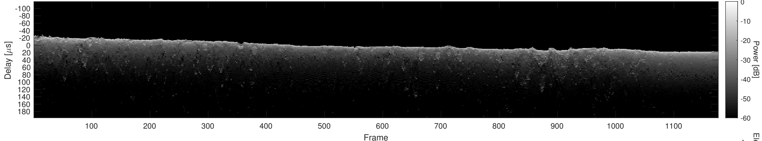
Orbit 12384, Cluttergram
