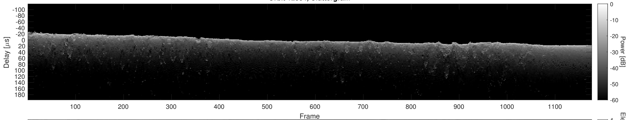
Orbit 12384, Cluttergram
