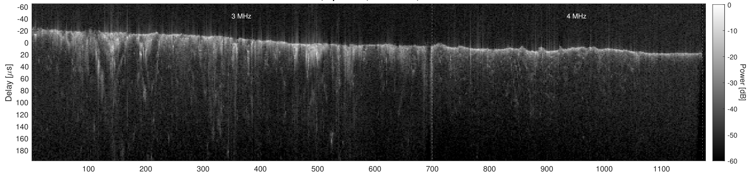
Orbit 12384, Cluttergram
