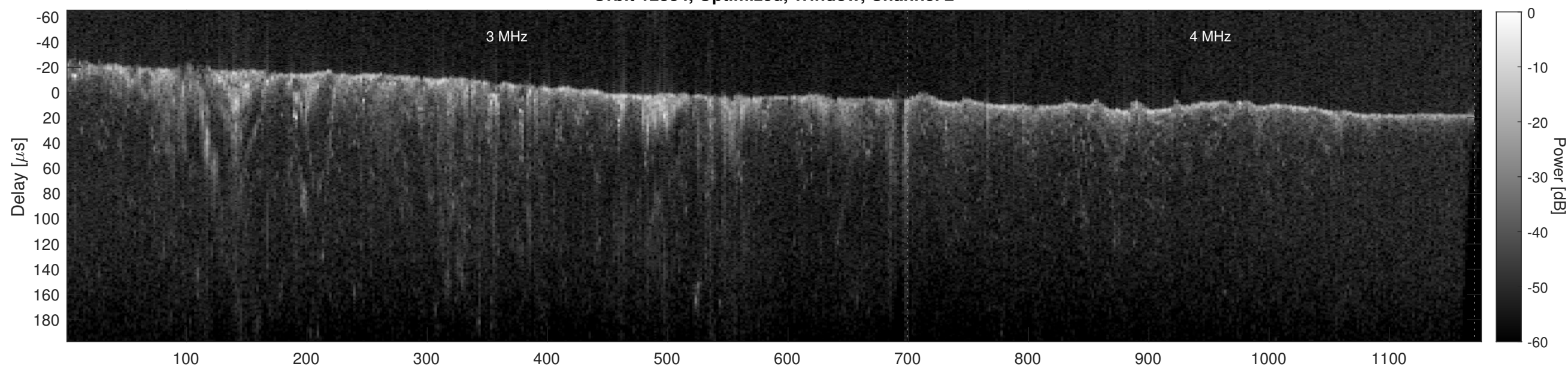
Orbit 12384, Cluttergram
