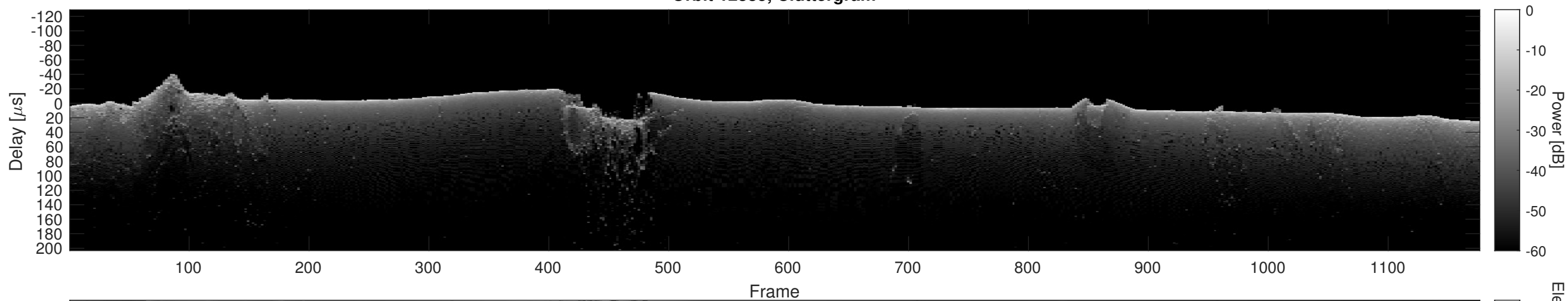
Orbit 12385, Cluttergram
