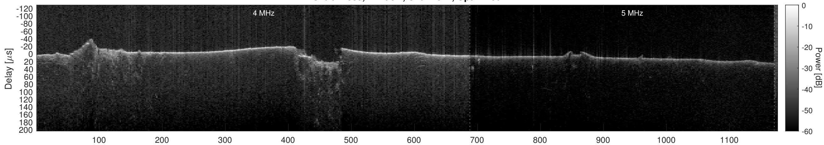
Orbit 12385, Cluttergram
