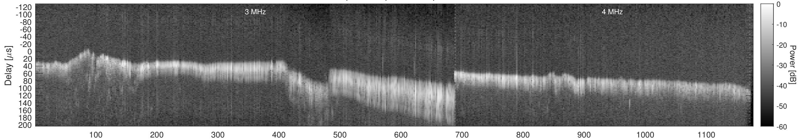
Orbit 12385, Window, Channel 2, Chapman
