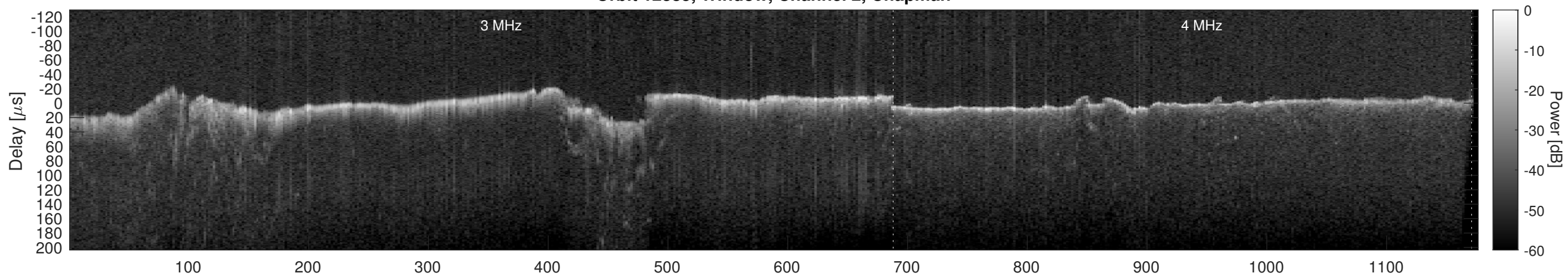
Orbit 12385, Window, Channel 2, Optimized
