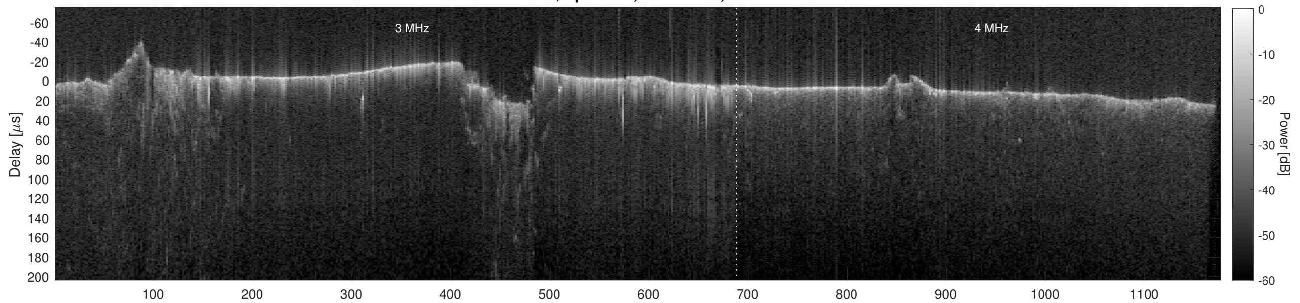
Orbit 12385, Cluttergram
