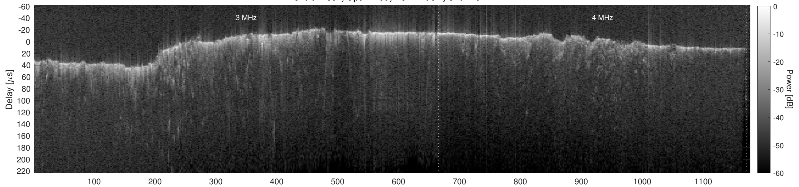
Orbit 12387, Cluttergram
