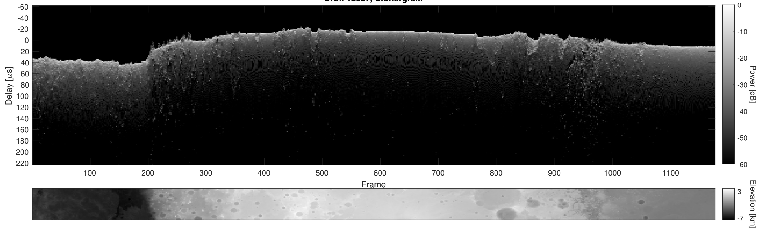
Orbit 12387, Cluttergram
