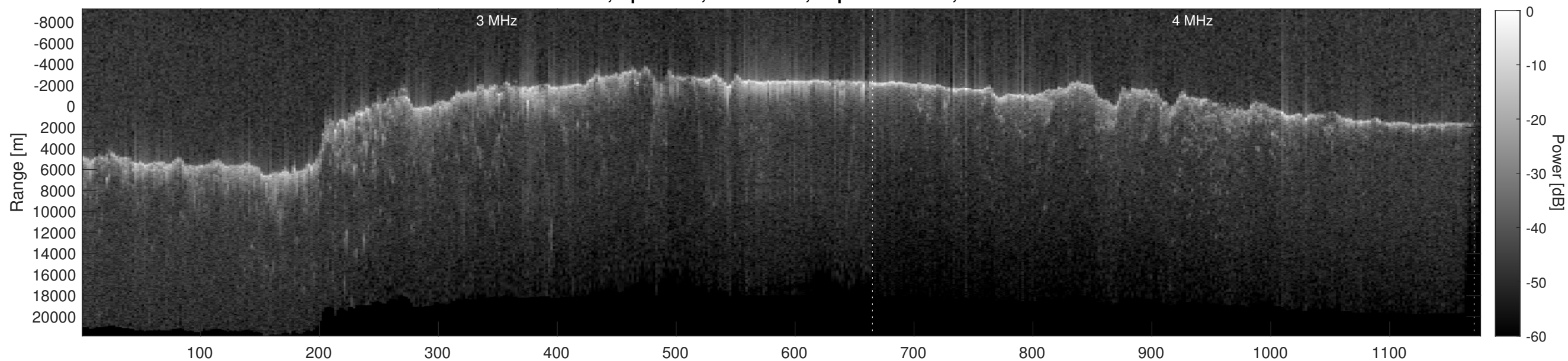
Orbit 12387, Depth-Corrected Cluttergram
