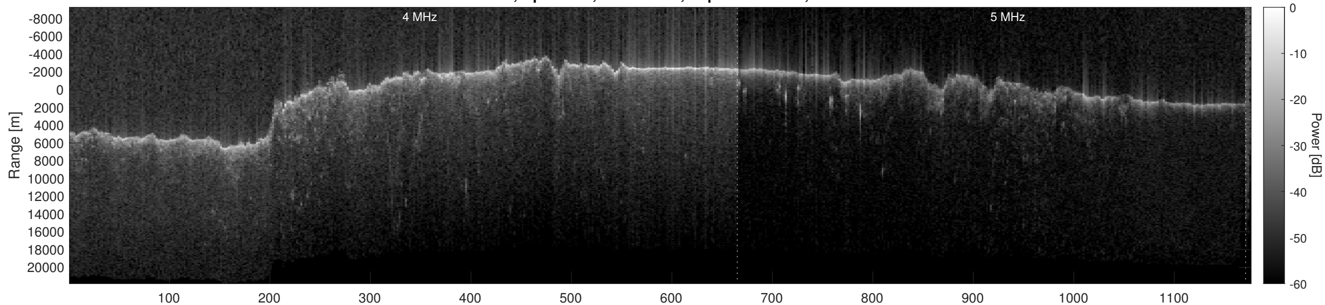
Orbit 12387, Optimized, No Window, Depth-Corrected, Channel 2
