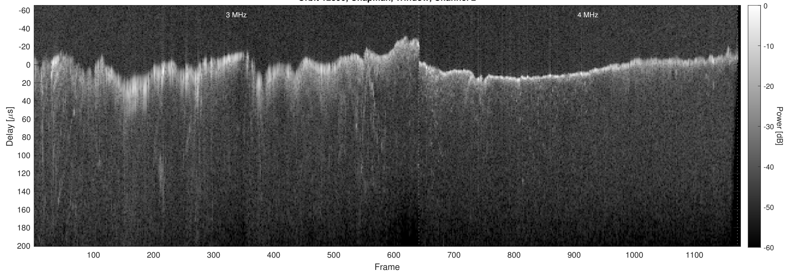
Orbit 12390, Chapman, Window, Channel 2
