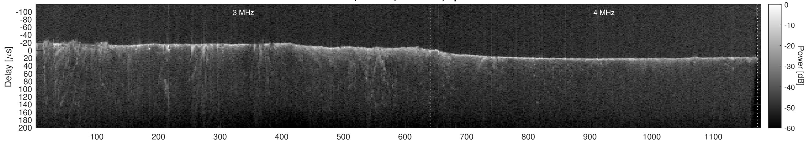
Orbit 12390, Cluttergram
