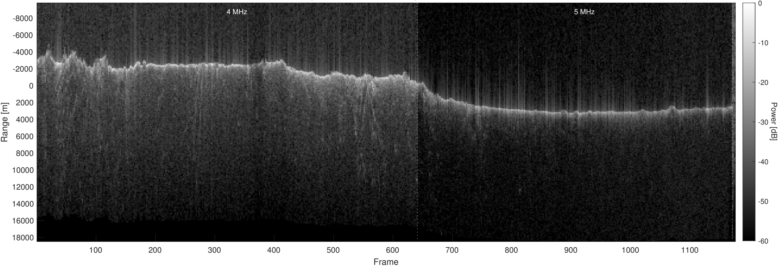
Orbit 12390, Optimized, No Window, Depth-Corrected, Channel 2
