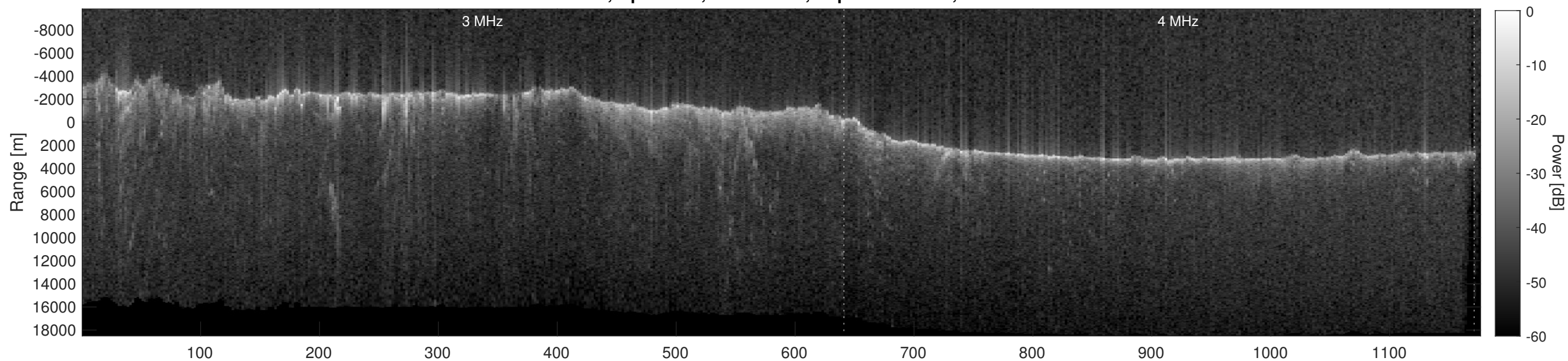
Orbit 12390, Depth-Corrected Cluttergram
