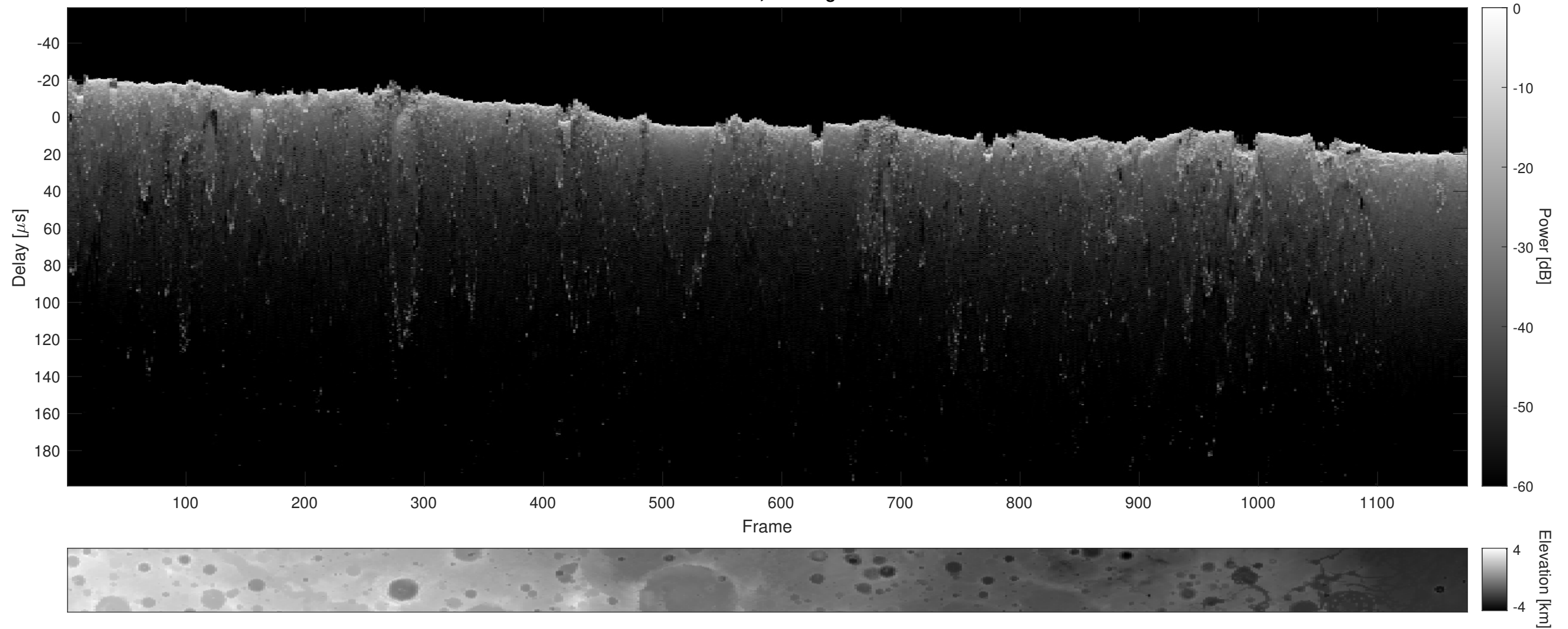
Orbit 12391, Cluttergram
