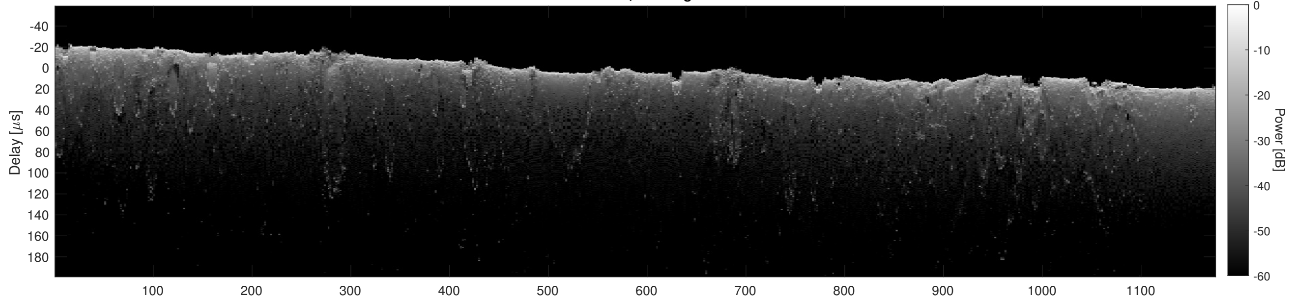
Orbit 12391, Cluttergram
