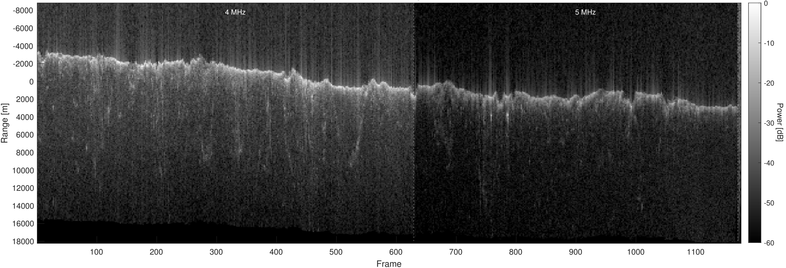
Orbit 12391, Optimized, No Window, Depth-Corrected, Channel 2
