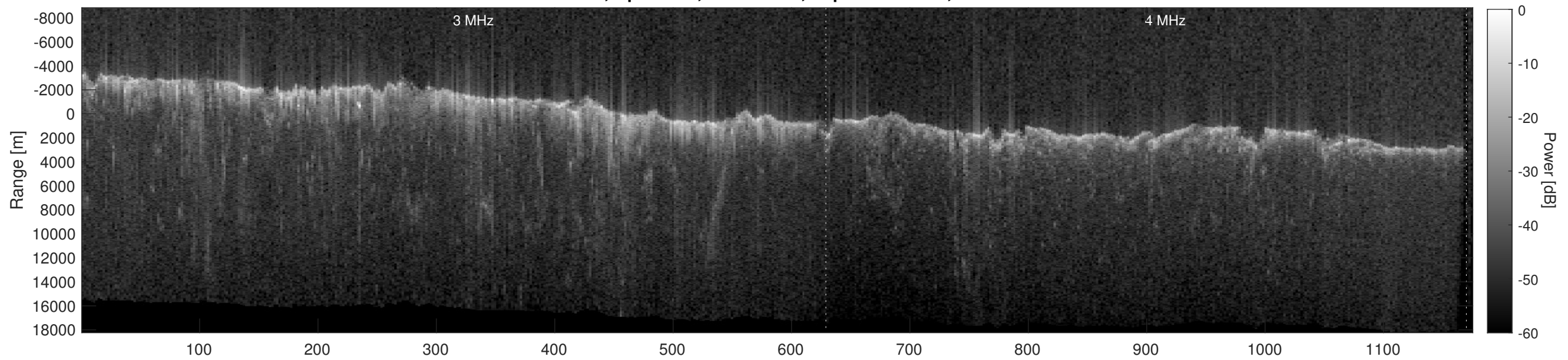
Orbit 12391, Depth-Corrected Cluttergram
