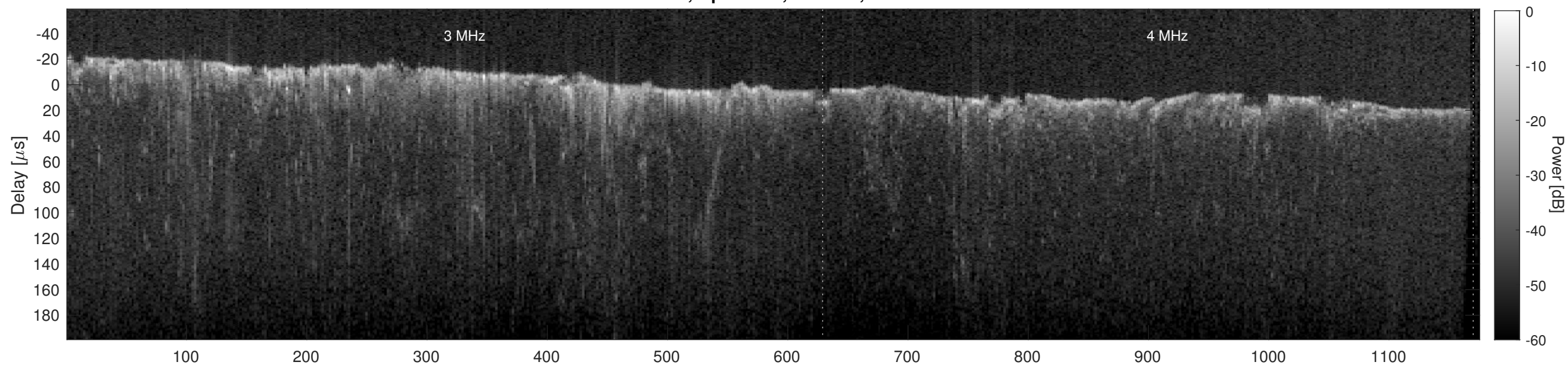
Orbit 12391, Cluttergram
