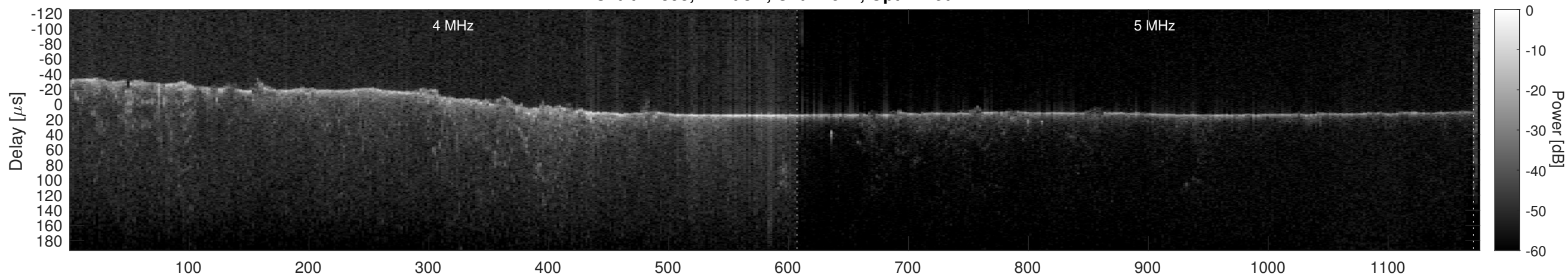
Orbit 12393, Cluttergram
