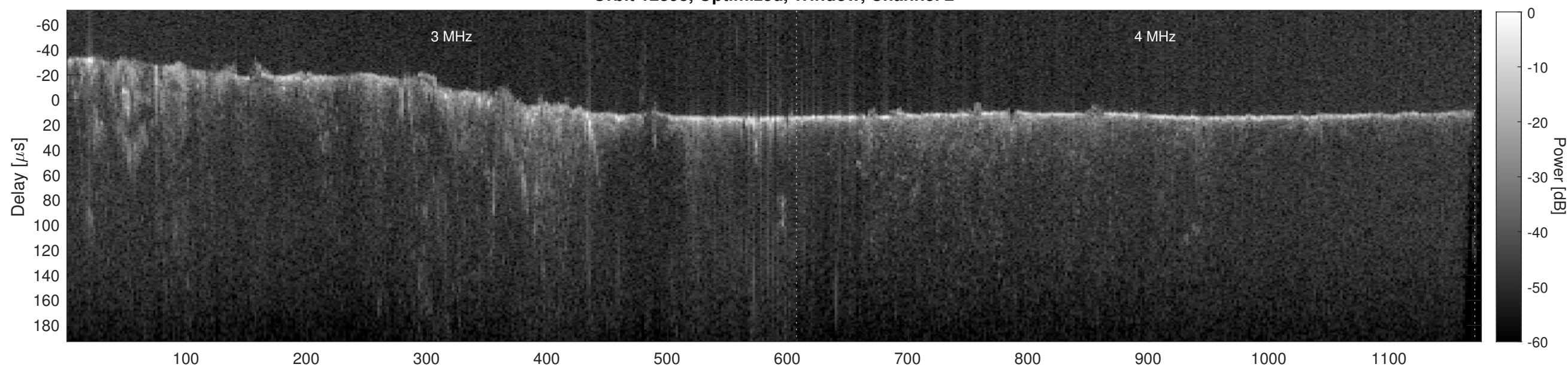
Orbit 12393, Cluttergram
