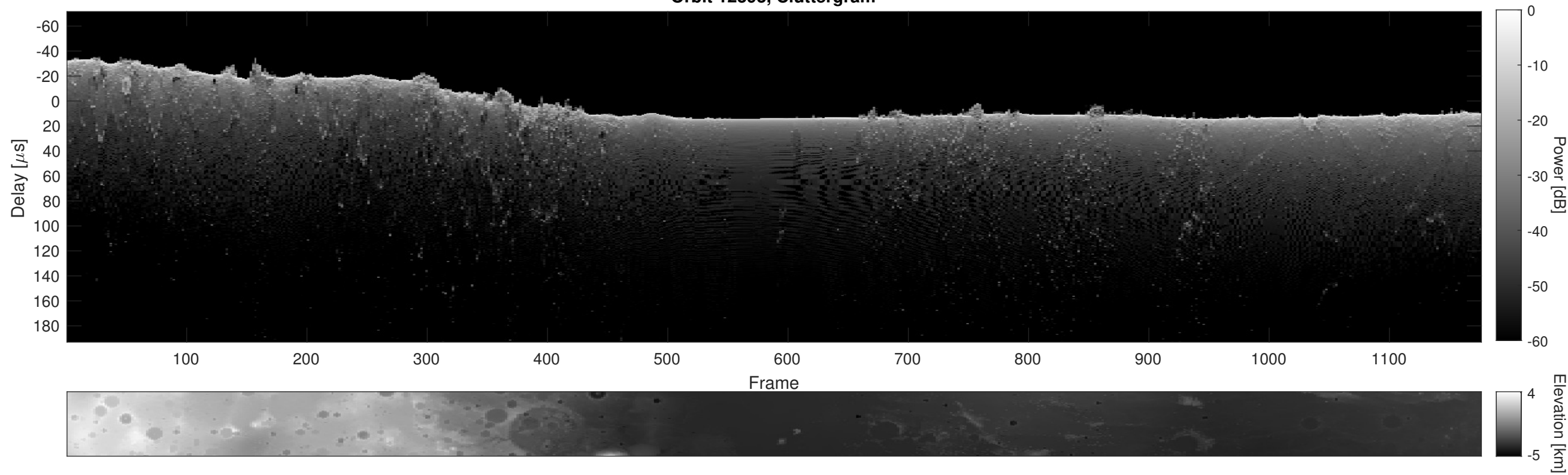
Orbit 12393, Cluttergram
