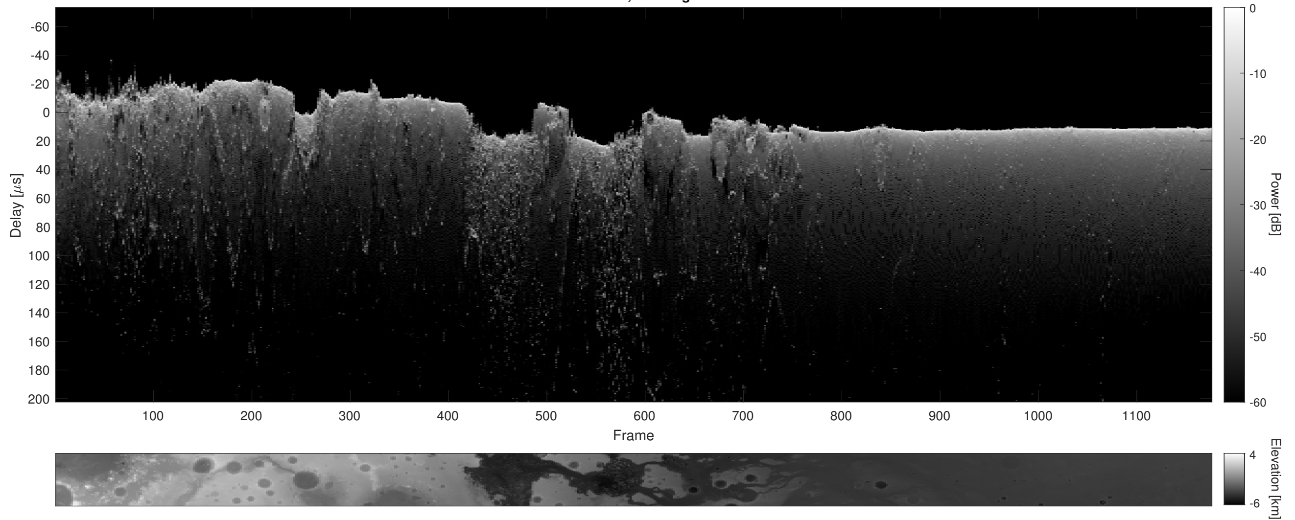
Orbit 12395, Cluttergram
