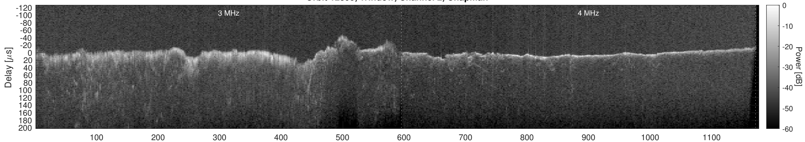
Orbit 12395, Window, Channel 2, Optimized
