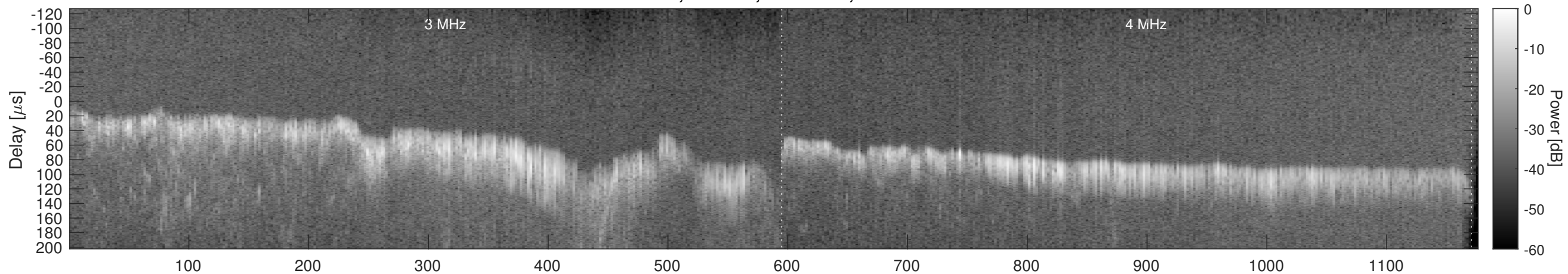
Orbit 12395, Window, Channel 2, Chapman
