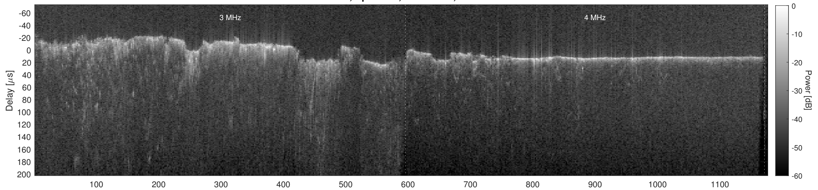
Orbit 12395, Cluttergram
