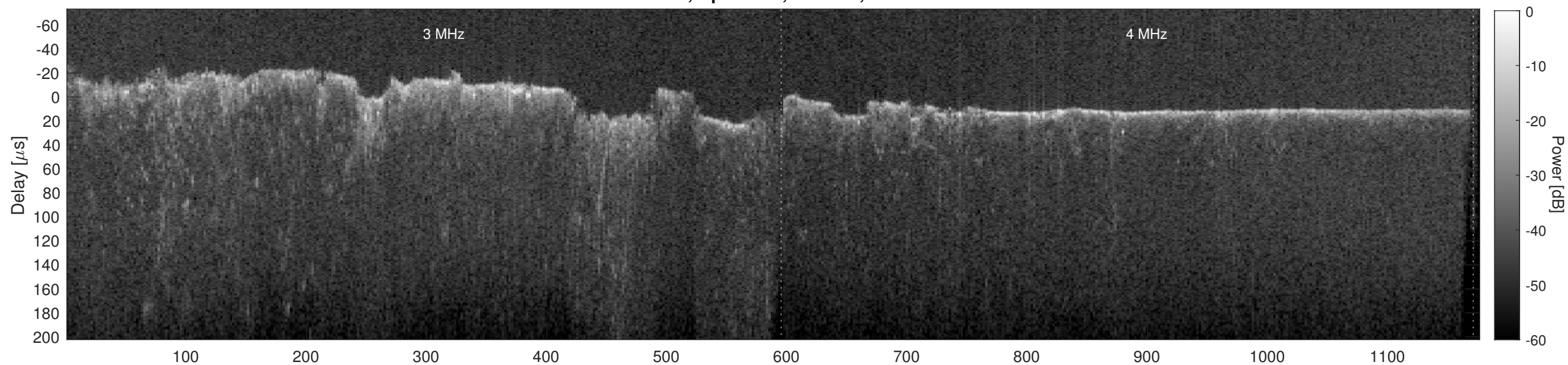
Orbit 12395, Cluttergram
