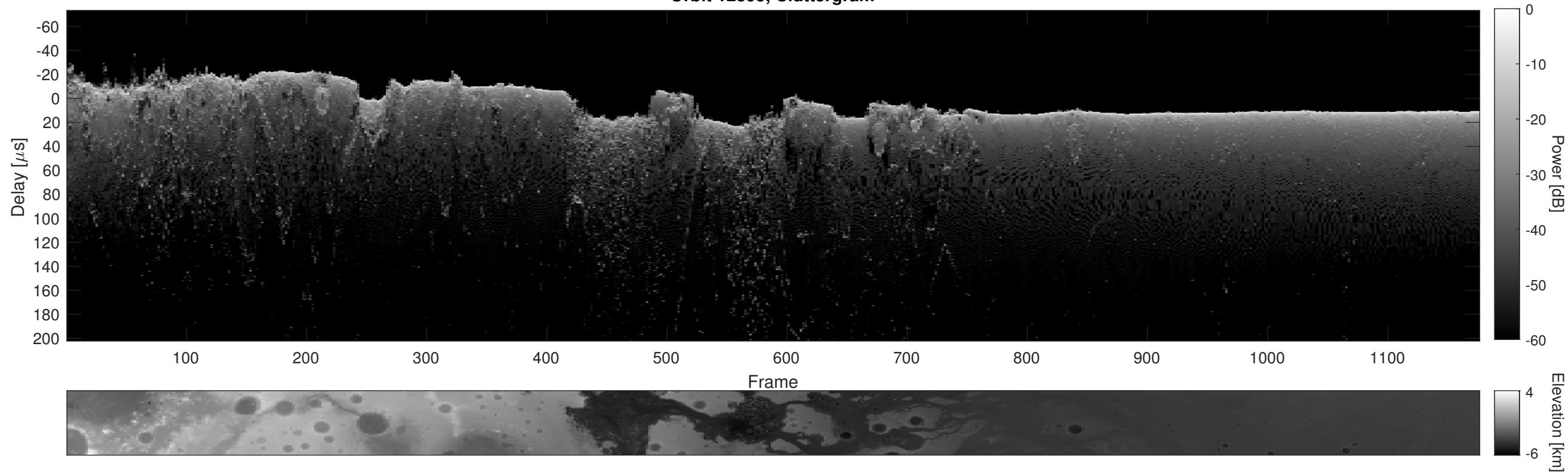
Orbit 12395, Cluttergram
