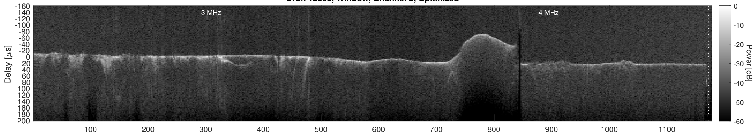
Orbit 12396, Cluttergram
