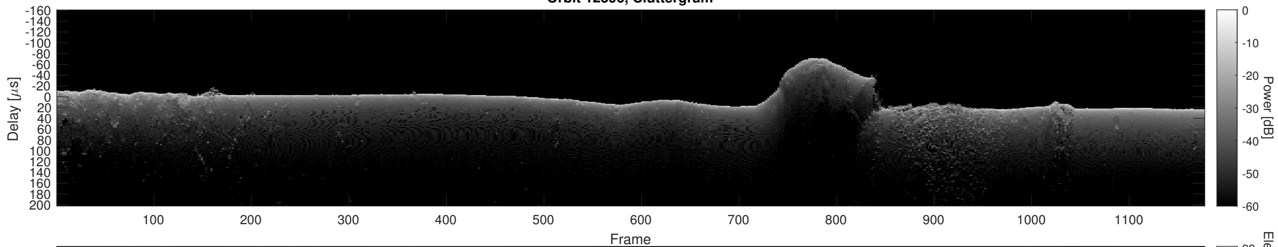
Orbit 12396, Cluttergram
