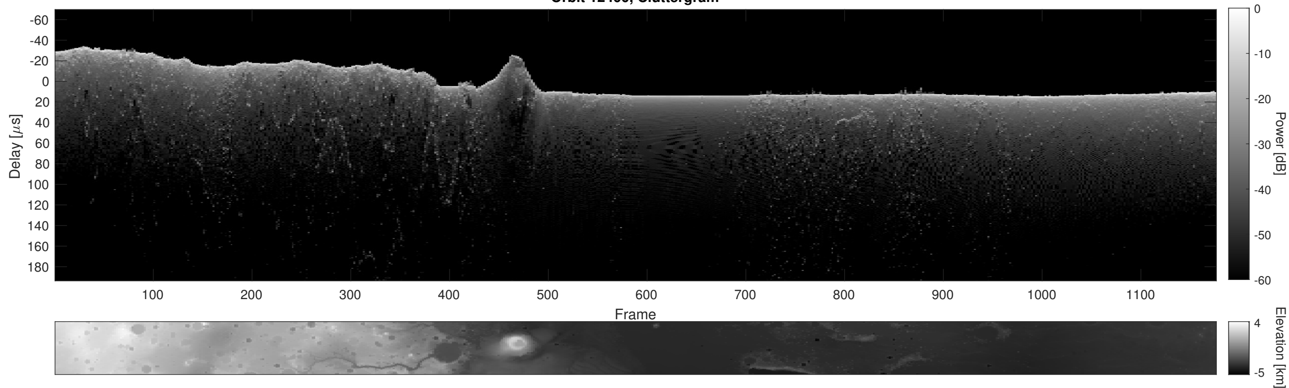
Orbit 12400, Cluttergram
