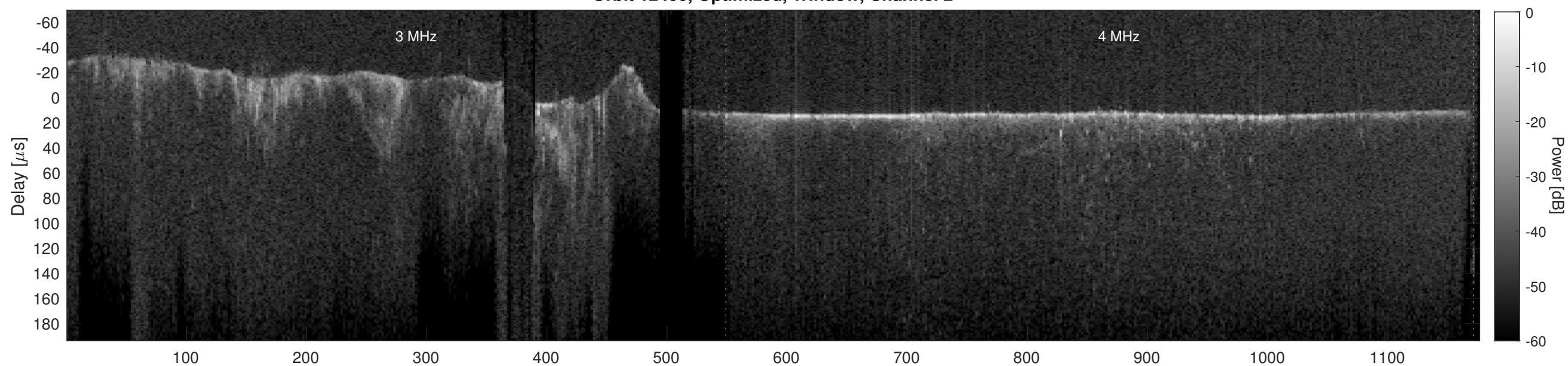
Orbit 12400, Cluttergram
