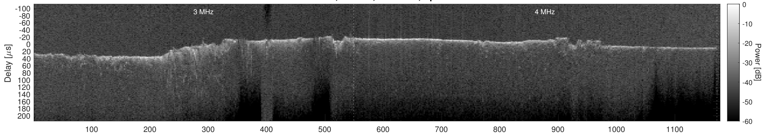
Orbit 12401, Cluttergram
