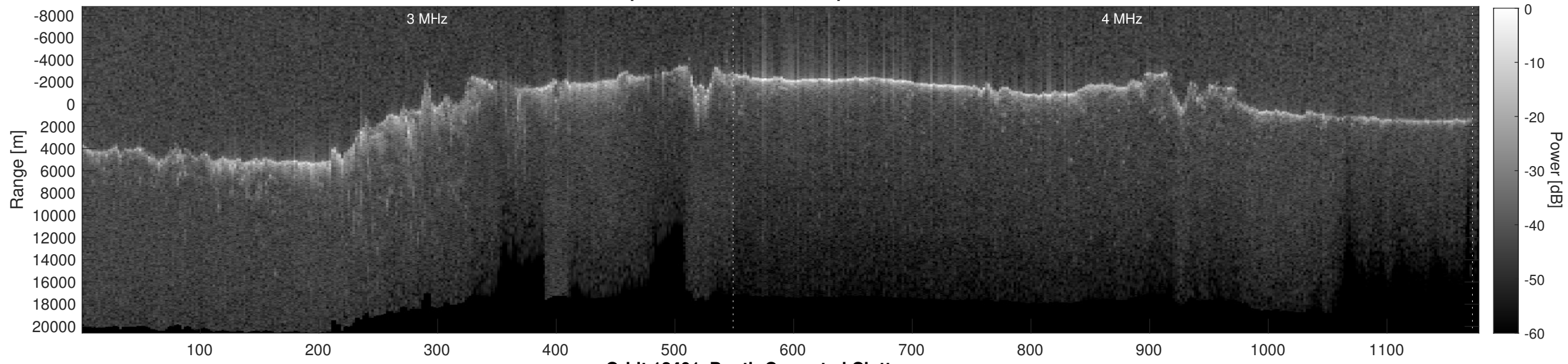
Orbit 12401, Depth-Corrected Cluttergram
