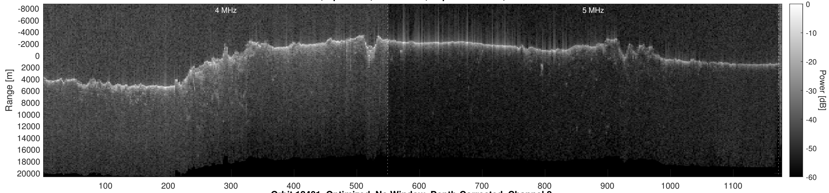
Orbit 12401, Optimized, No Window, Depth-Corrected, Channel 2
