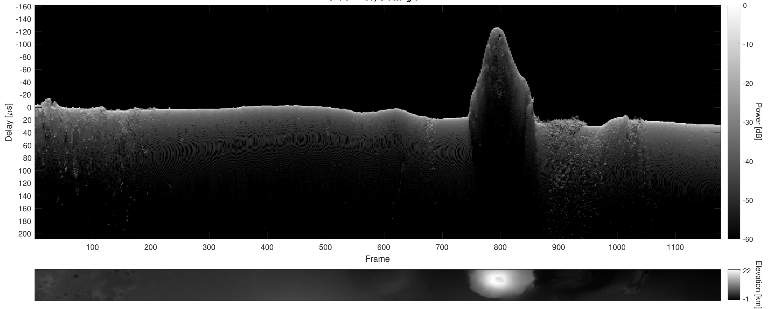
Orbit 12403, Cluttergram
