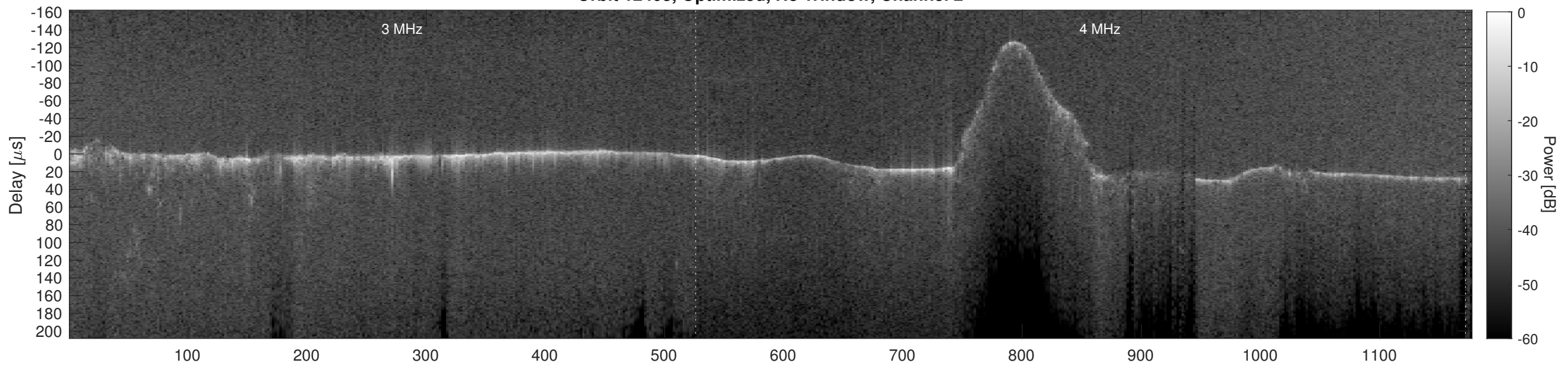
Orbit 12403, Cluttergram
