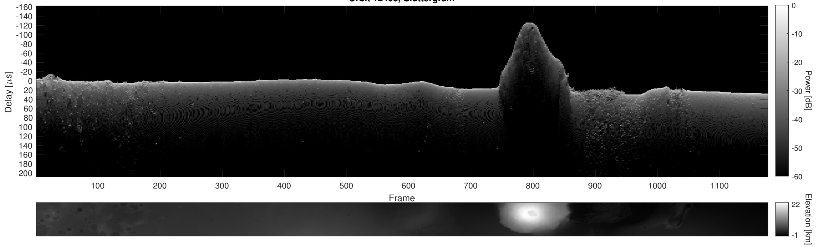
Orbit 12403, Cluttergram
