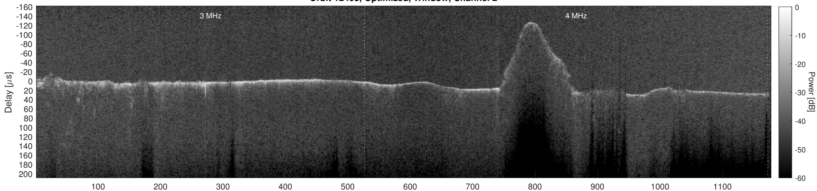
Orbit 12403, Cluttergram
