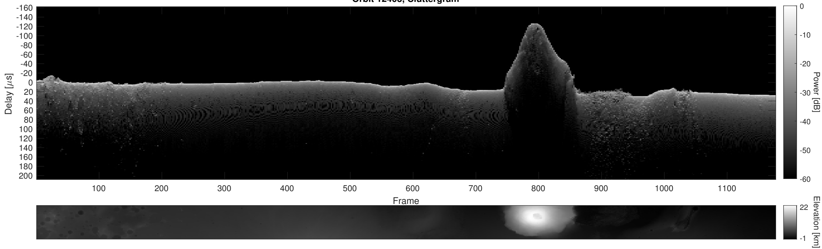
Orbit 12403, Cluttergram
