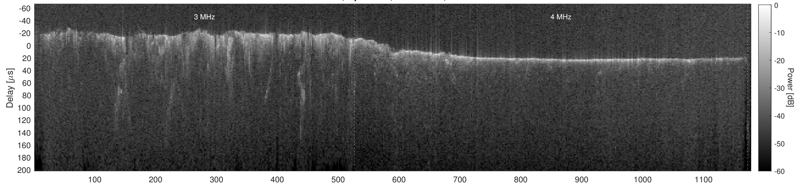
Orbit 12404, Cluttergram
