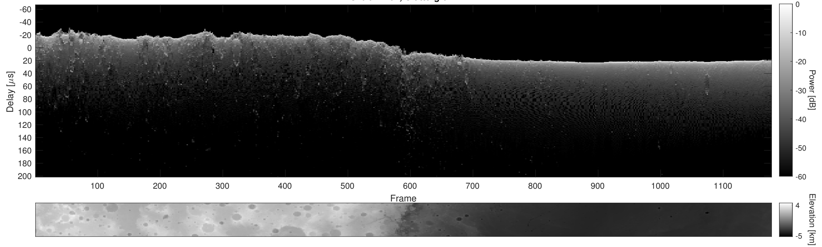
Orbit 12404, Cluttergram
