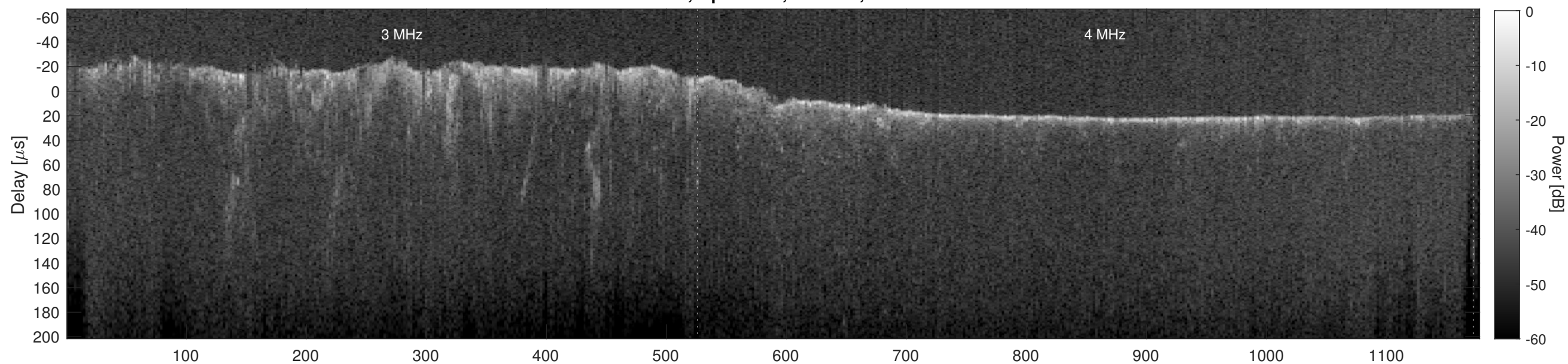
Orbit 12404, Cluttergram
