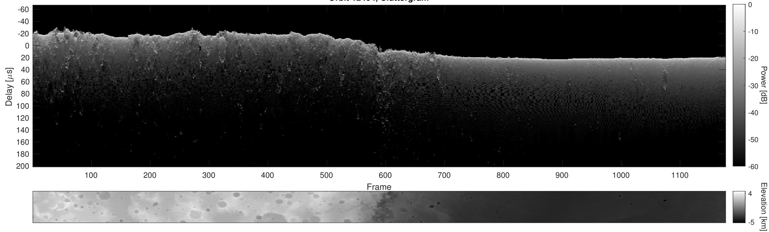
Orbit 12404, Cluttergram
