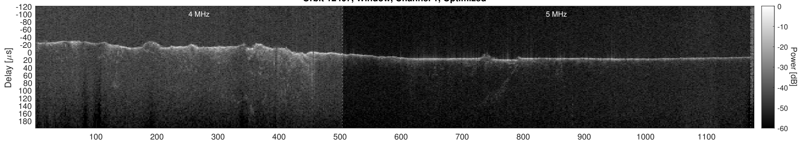
Orbit 12407, Cluttergram
