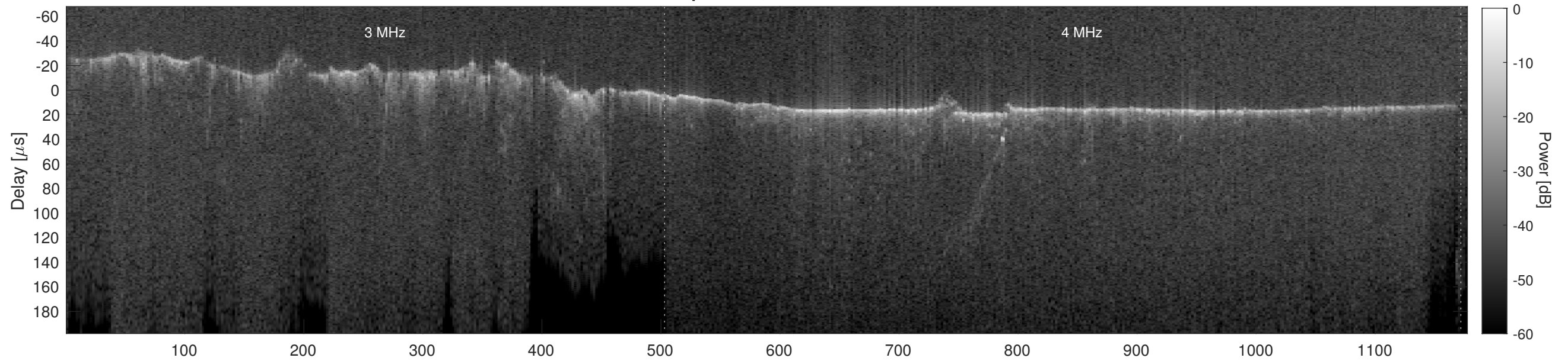
Orbit 12407, Cluttergram
