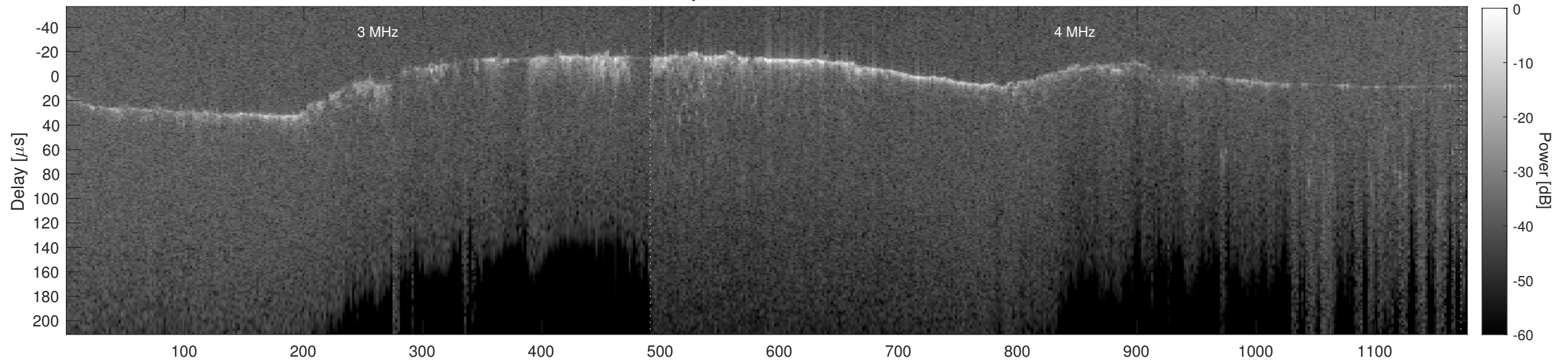
Orbit 12408, Cluttergram
