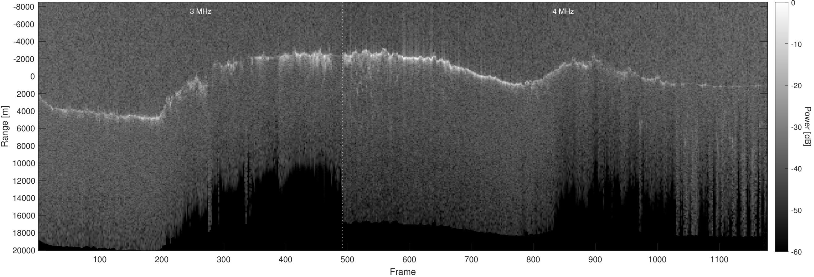
Orbit 12408, Optimized, No Window, Depth-Corrected, Channel 2
