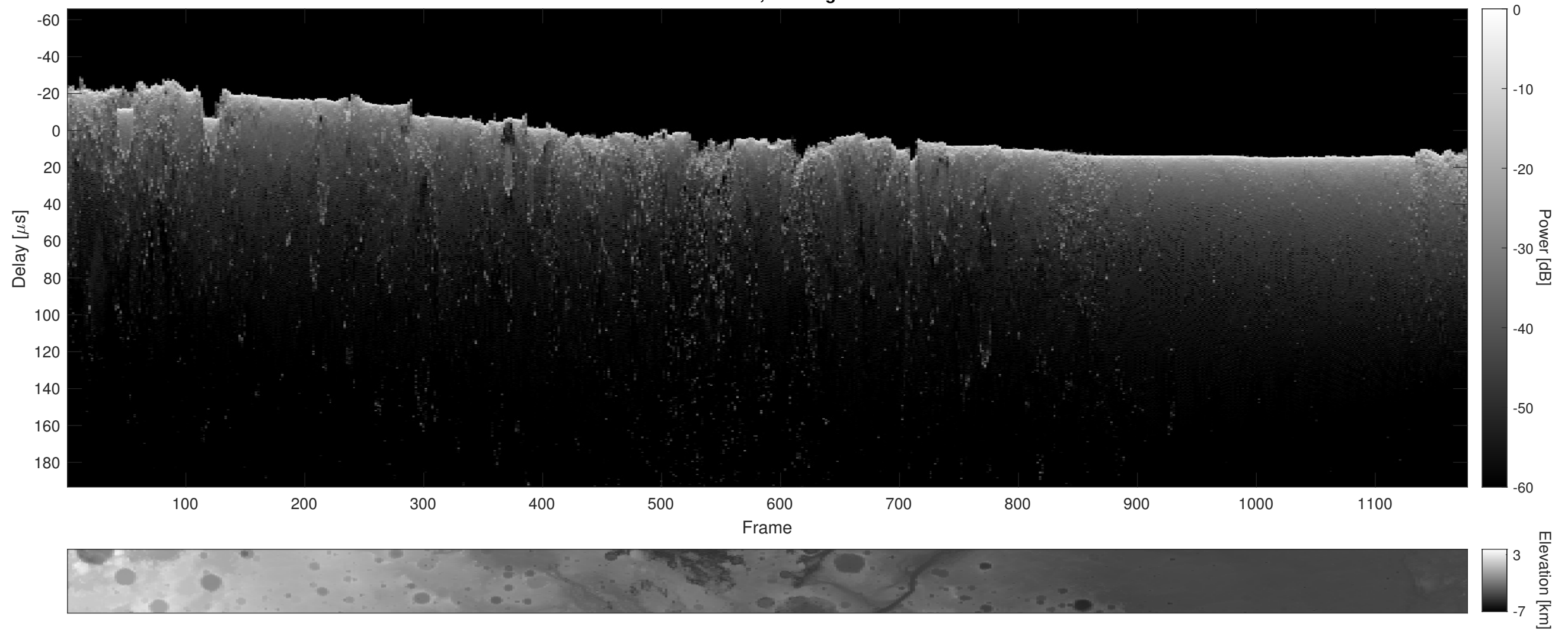
Orbit 12409, Cluttergram
