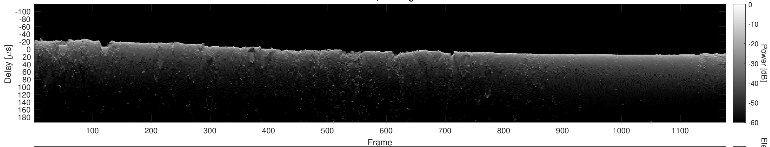
Orbit 12409, Cluttergram
