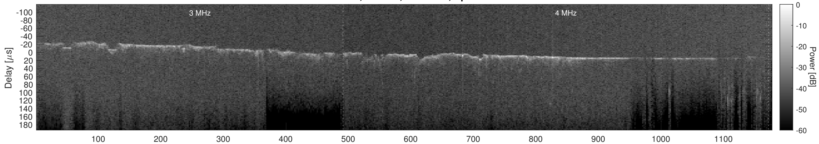
Orbit 12409, Cluttergram
