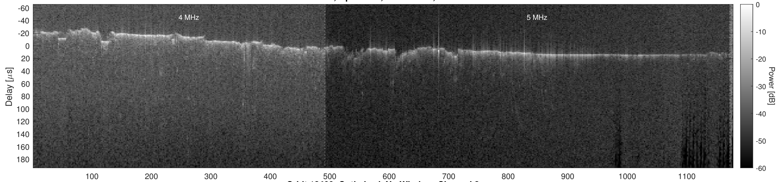
Orbit 12409, Optimized, No Window, Channel 2
