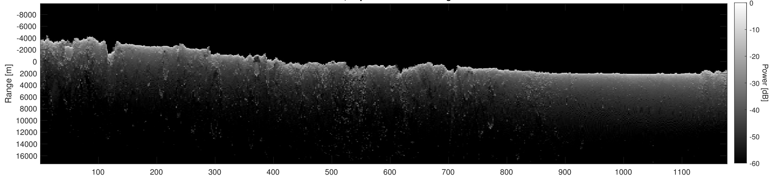
Orbit 12409, Depth-Corrected Cluttergram
